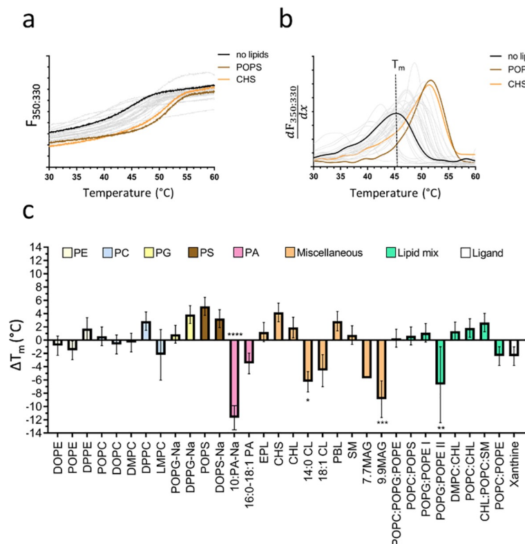
Fig 2. Lipid screening of UapA by nanoDSF. (a) F_{350:330} signal of the no lipids reference sample (black line) and a representative set of stabilising lipids (coloured lines) during the melting scan. Grey lines show the fluorescence traces of the other tested lipids. (b) First derivative of the F_{350:330} signal highlighting the fluorescence change indicative of protein unfolding. The T_m can be determined at the curve peak, here shown for the no lipids reference sample as dotted line. (c) \Delta T_m of detergent-solubilised to relipidated sample shown for all tested lipids, which are sorted and colour coded according to their lipid class. Panel a-b show the traces of a representative nanoDSF scan. Panel c shows the \Delta T_m and corresponding SEM based on three technical repeats. The asterisks represent the p-value (* = 0.0332, ** = 0.021, *** = 0.002, **** = 0.0001) obtained by a one-way ANOVA followed by a Dunnett test to correct for multiple comparison in GraphPadPrism 7.
